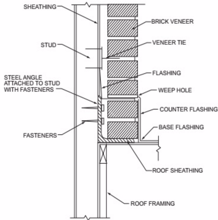
SUPPORT BY STEEL ANGLE
