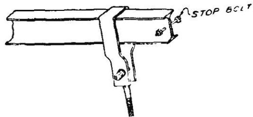
Suspended Scaffold—Thrustout.
